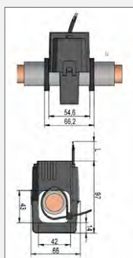
SC 50-E
